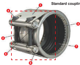
Standard coupling
