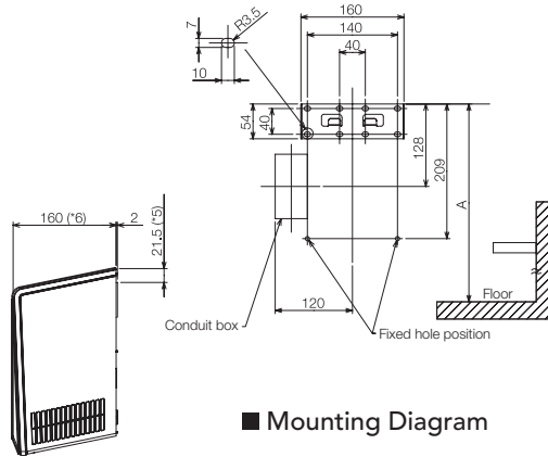
Bracket height recommendation
