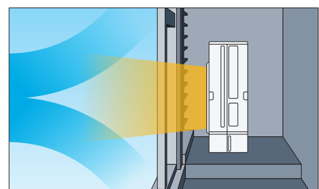
30Pa external static pressure fan motor (option) (PAC-SJ71FM-E)
