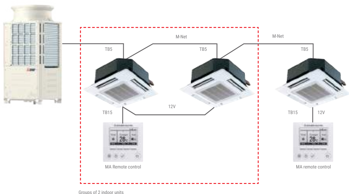
EXAMPLE OF WIRED CONNECTION (MA controller)
