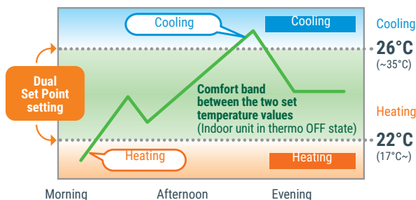
EXAMPLE OF USAGE OF HIGH SENSIBLE HEAT OPERATION FUNCTION WITH MULTIPLE HUMIDITY SENSORS
