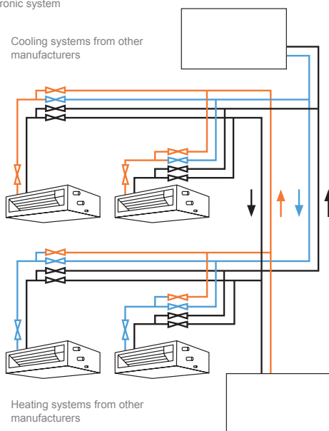
Traditional 4-pipe hydronic system
