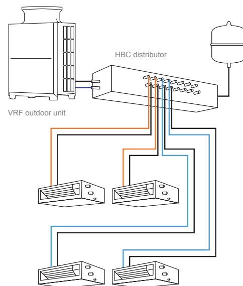
Hydronic CITY MULTI 2-pipe system
