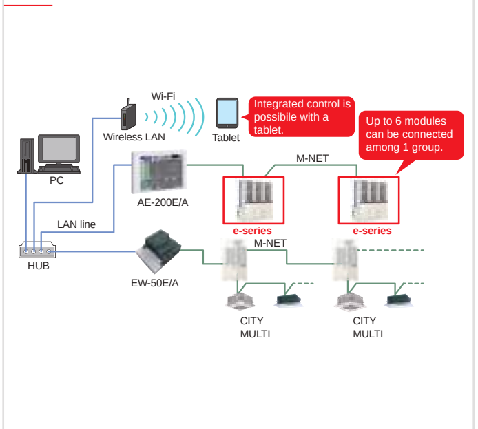
SYSTEM CONFIGURATION AE-200E/A
