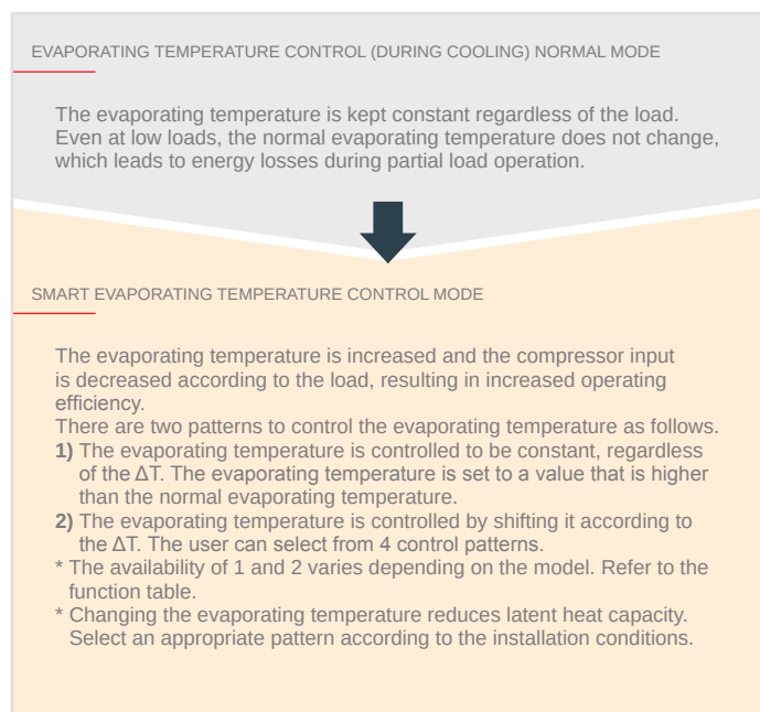
2) EVAPORATING TEMPERATURE CONTROL IMAGE (WITH 4 PATTERNS)
