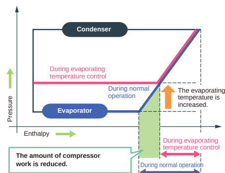
1) EVAPORATING TEMPERATURE CONTROL IMAGE
