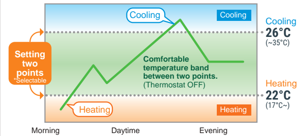
OPERATION PATTERN DURING AUTO (DUAL SET POINT) MODE
