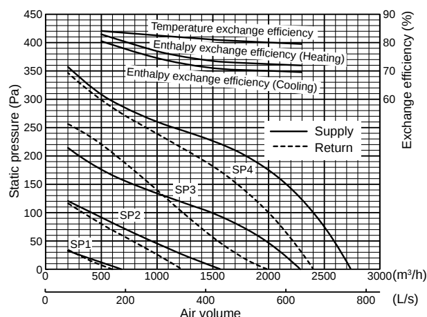
Characteristic Curve of the LGH-200RVXT-E
