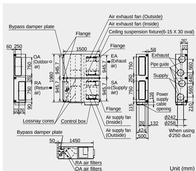
Dimensions of the LGH-150RVXT-E
