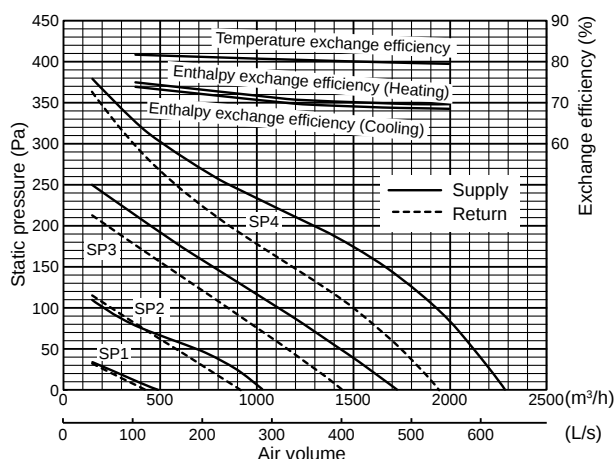
Characteristic Curve of the LGH-150RVXT-E
