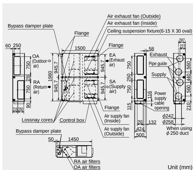
Dimensions of the LGH-200RVXT-E
