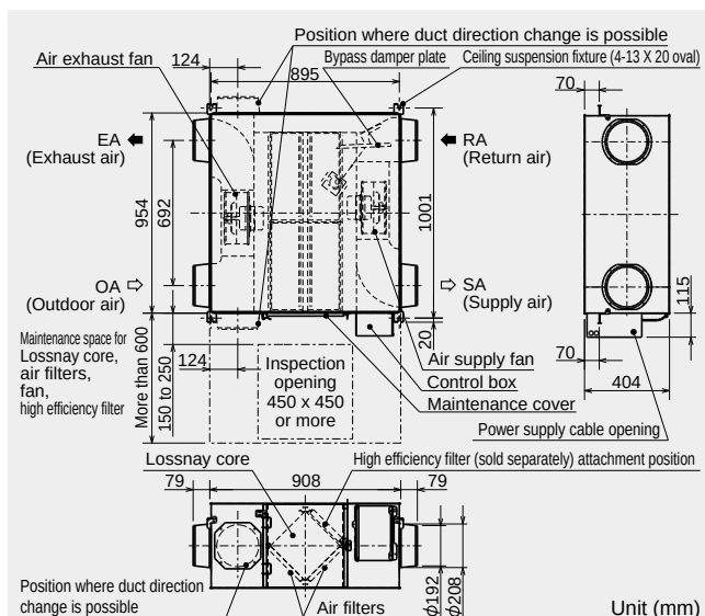
Dimensions of the LGH-65RVX-E
