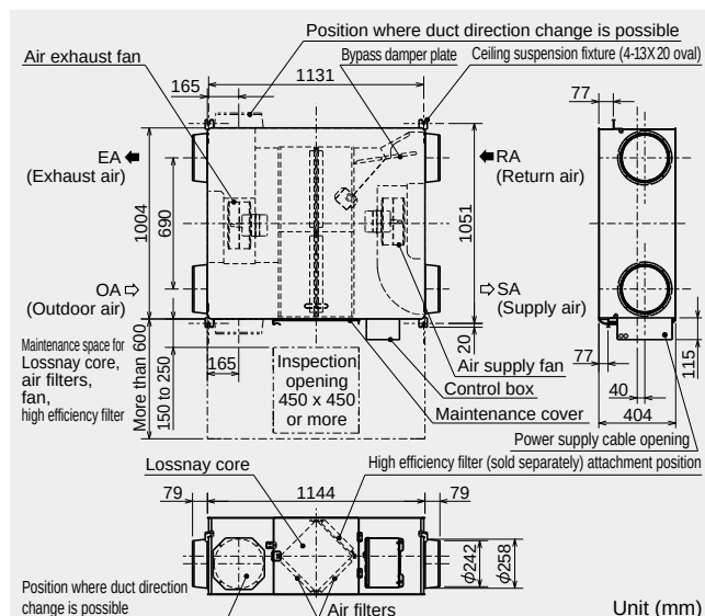
Dimensions of the LGH-80RVX-E
