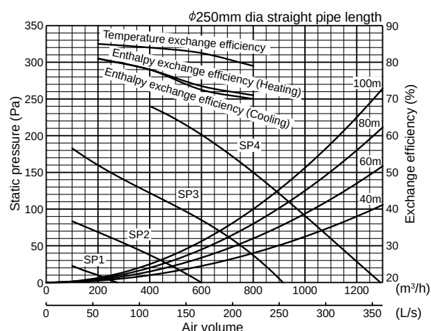
Characteristic Curve of the LGH-80RVX-E
