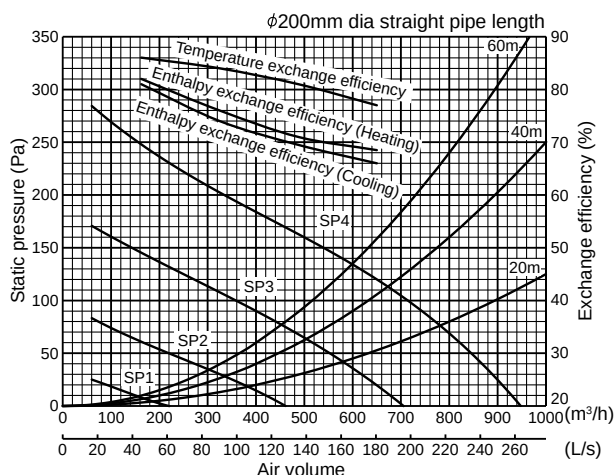
Characteristic Curve of the LGH-65RVX-E
