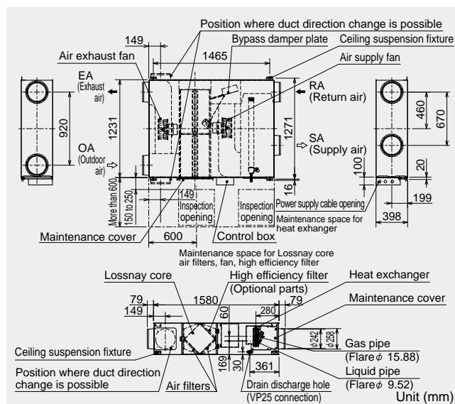
Dimensions of the GUF-100RD4
