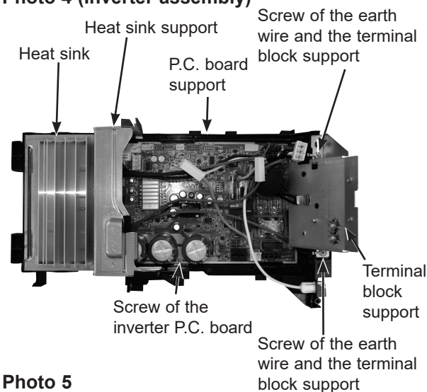
Photo 4 (Inverter assembly)
