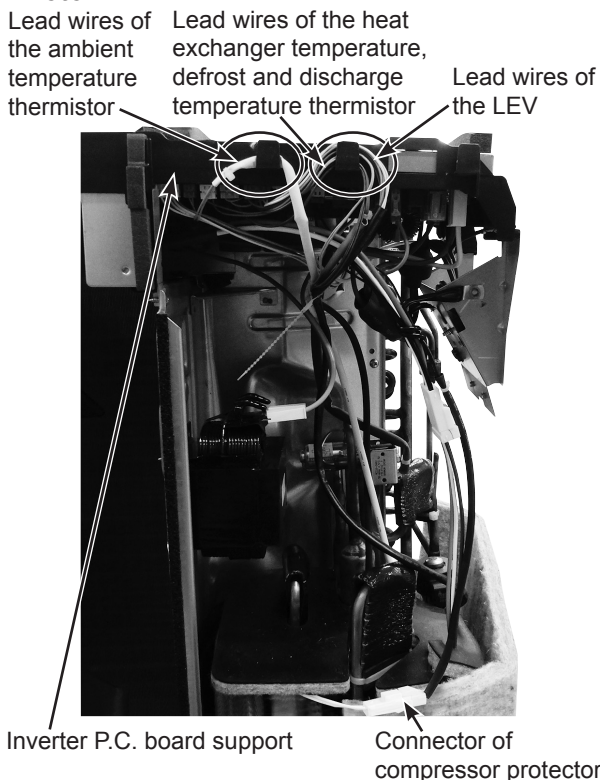
Photo 5 (Inverter assembly)
