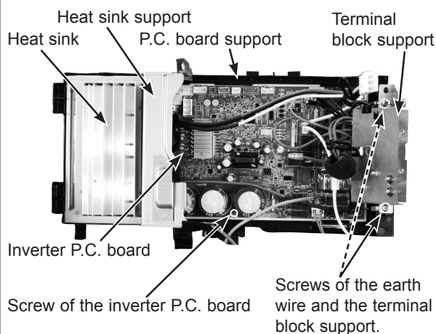
Photo 5 (Inverter assembly)
