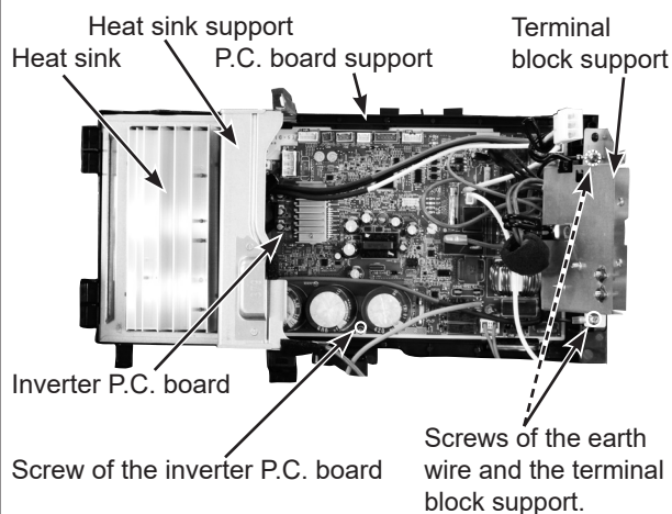
Photo 5 (Inverter assembly)
