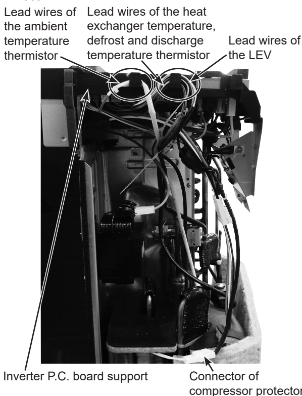
Photo 5 (Inverter assembly)
